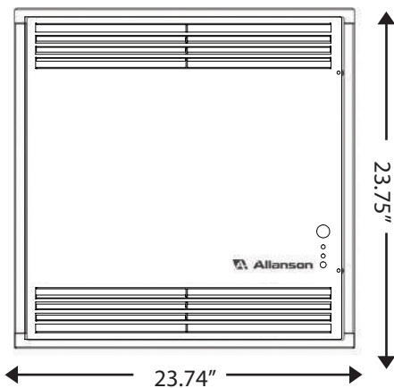
UVC Ceiling Fixture Front View
