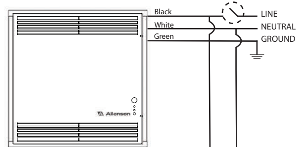
Multiple Unit Connection with Optional Wall Switch
