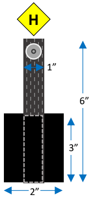
Qty 1 Upper Right Torso 1" x 16" Webbing 2" x 3" Hook Qty 1 Female Snap.
