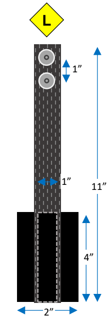
Qty 2 Thigh 1" x 11" Webbing 2" x 4" Hook Qty 2 Female Snaps.
