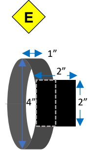
Qty 2 Hand Plate Strap 1" x 8" Elastic Loop 2" x 2" Hook
