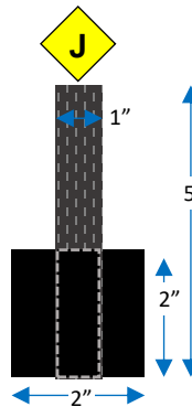
Qty 2 Built into Kidney Plate 1" x 5" Webbing 2" x 2" Hook On Part #06.
