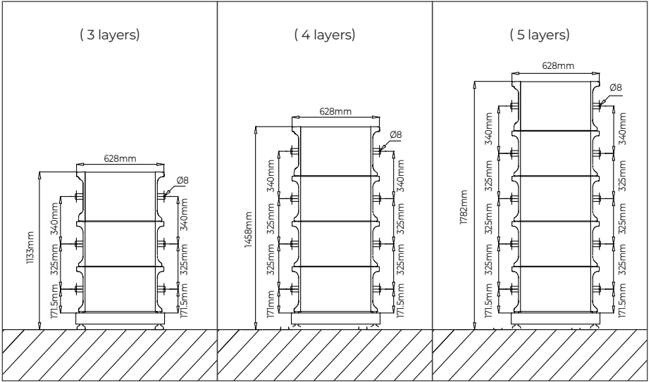
Figure 5-3 (Unit: mm)
