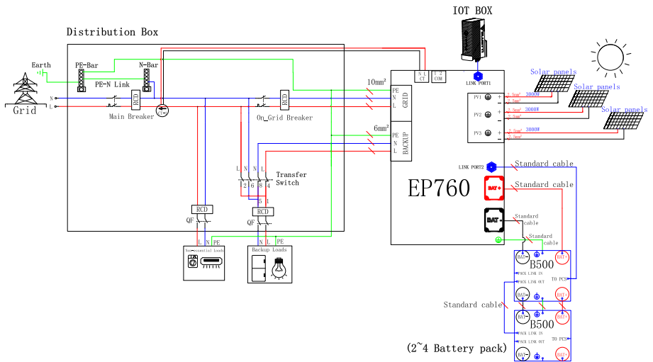
Figure 5-15 DC Coupling
