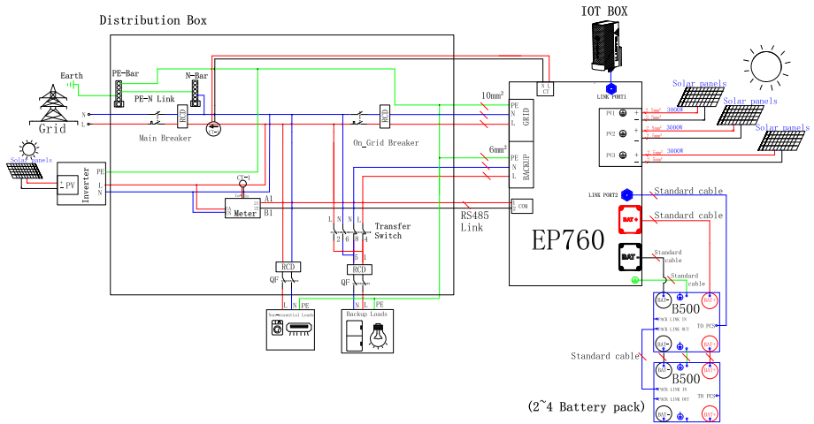
Figure 5-16 AC Coupling
