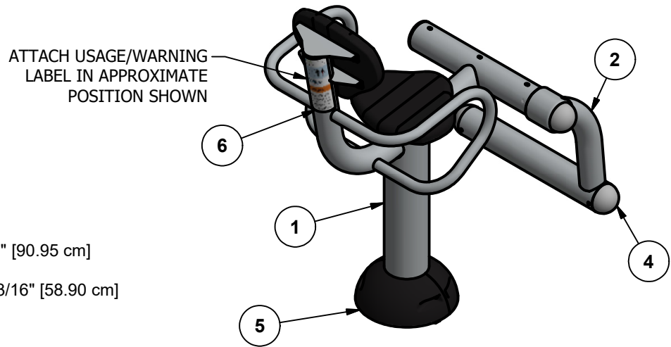
ASSEMBLY DRAWINGS
