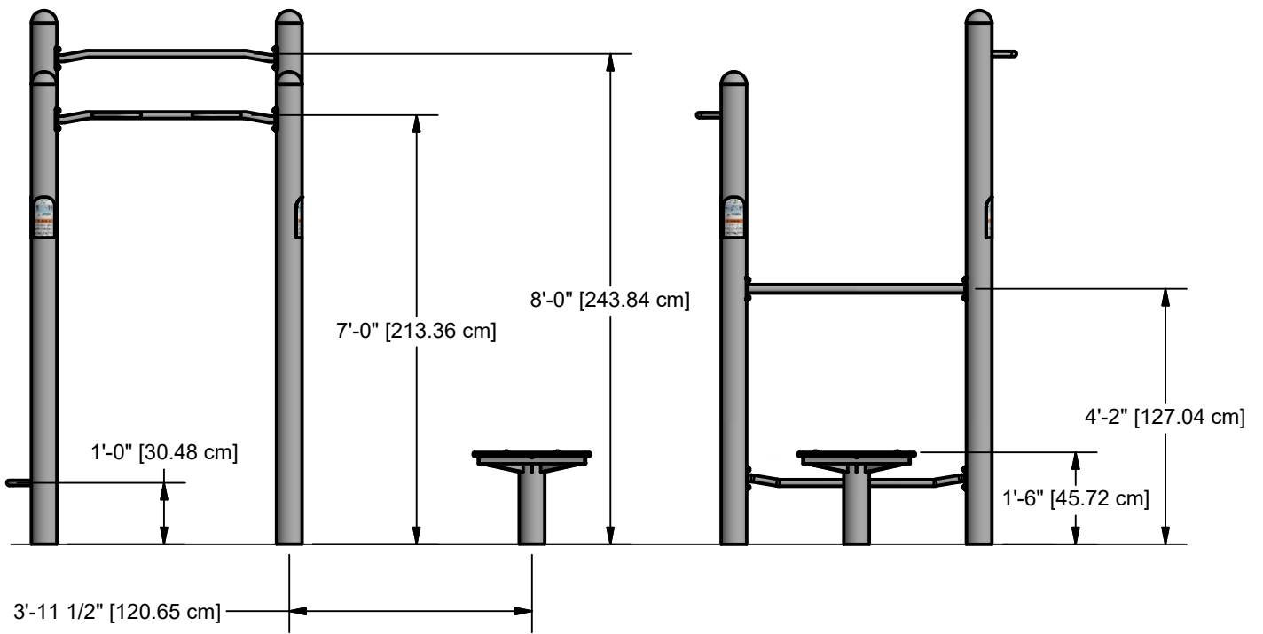
FRONT & SIDE ELEVATION VIEWS
