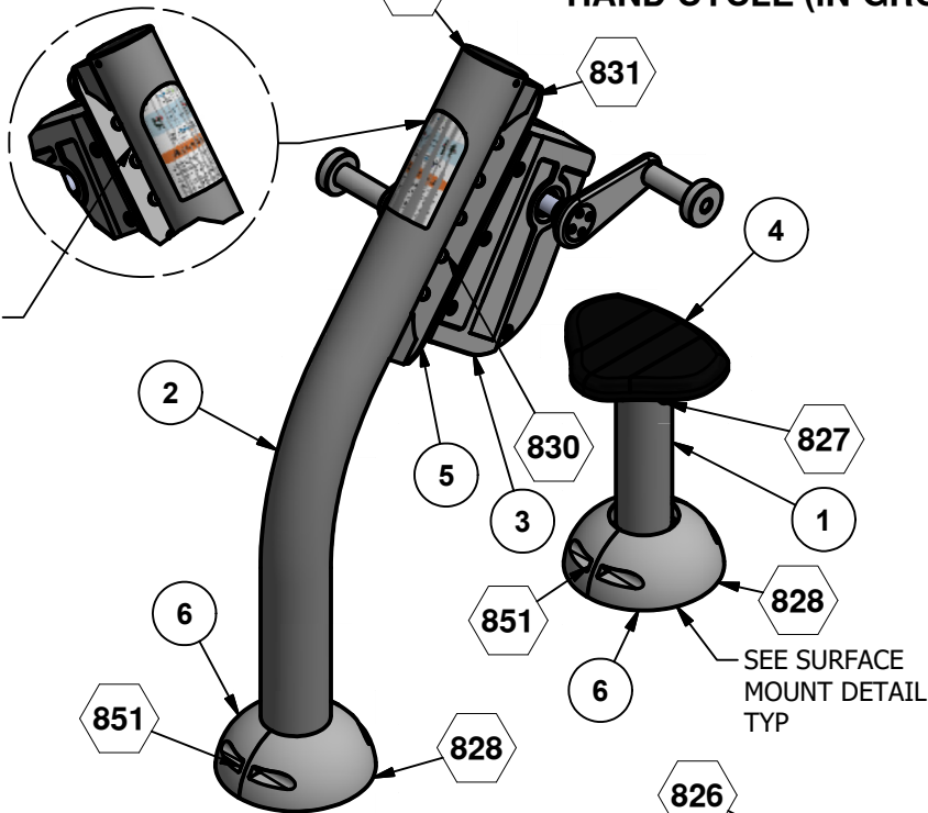
ASSEMBLY DRAWING UP216SM
