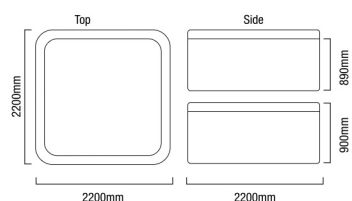
Structure Frame drawing of POLARIS
