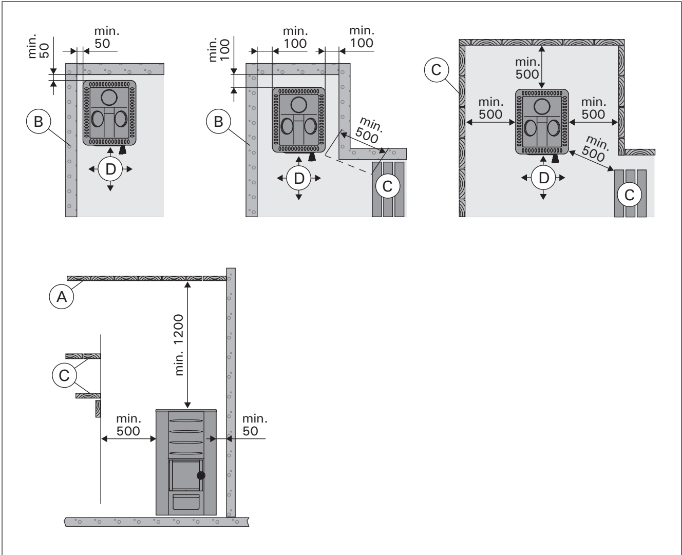
Safety distances (all dimensions in millimeters)
