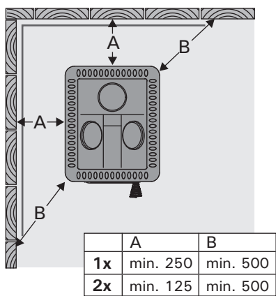
Protective covers (all dimensions in millimeters)
