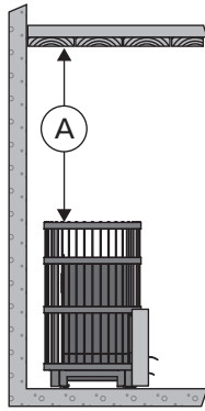
Safety distances (all dimensions in millimeters)
