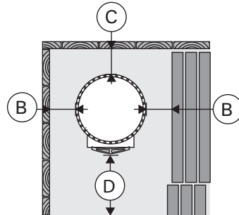
Safety distances (all dimensions in millimeters)
