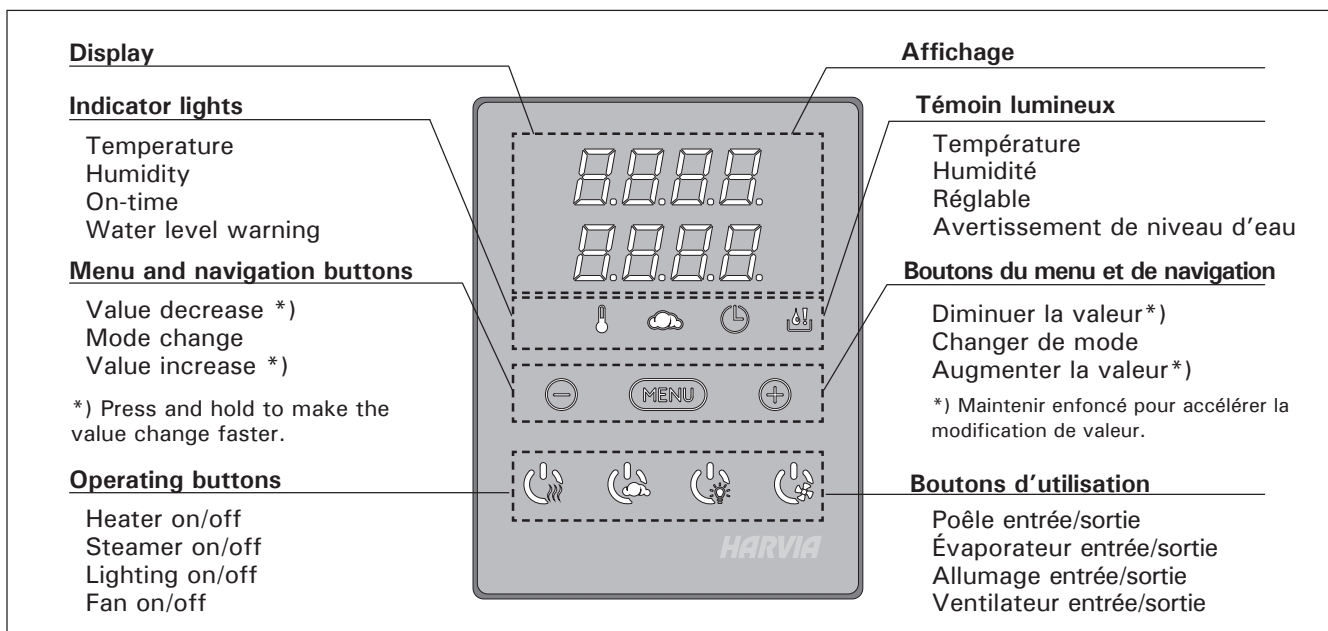
Figure 2. Control panel
