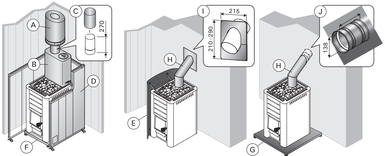
Accessories (all dimensions in millimeters)
