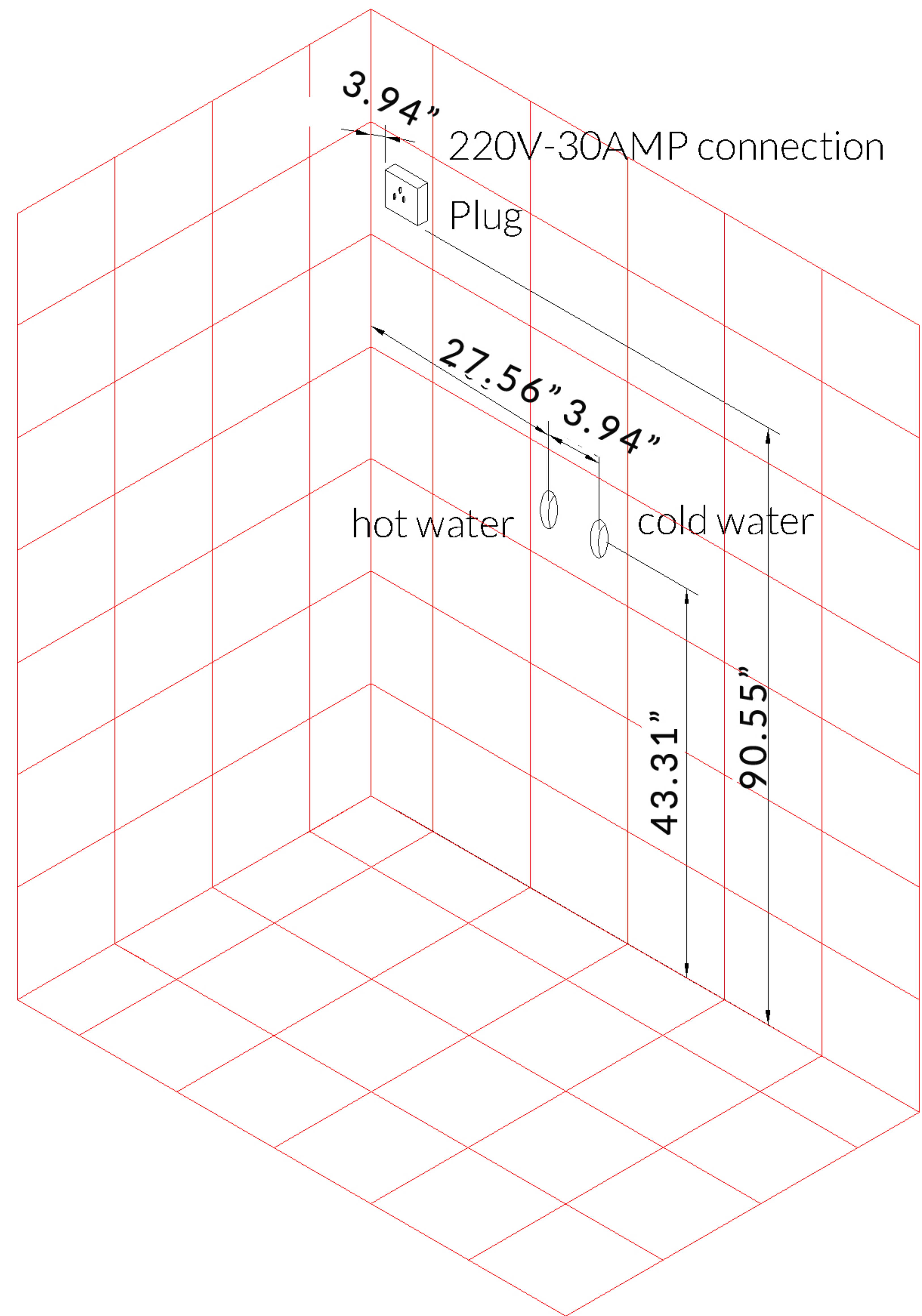
DZ972-3F8 INSTALLATION DIMENSIONS: 59" x 35" x 87"
