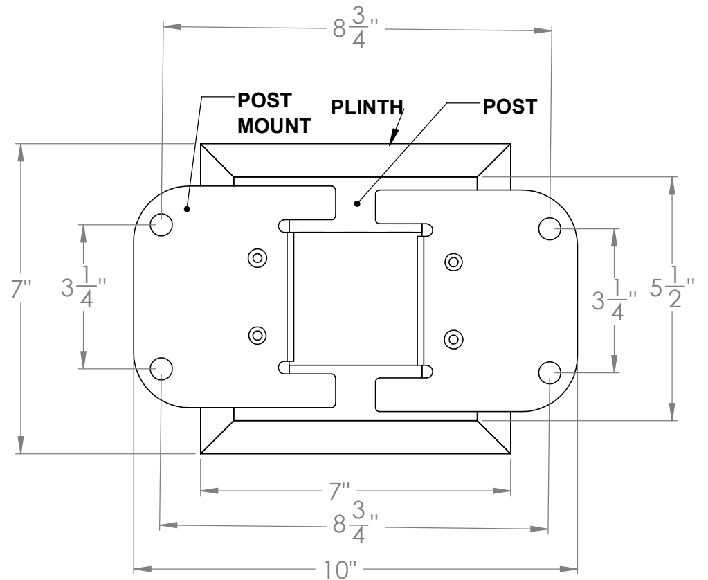
POST DETAIL
