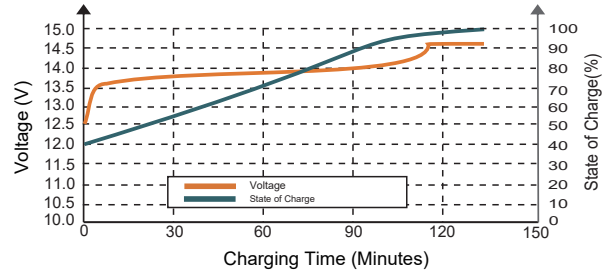
STATE OF CHARGE CURVE (0.5C, 25°C)
