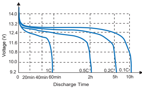
Discharge Curve at Different Rates (25°C)
