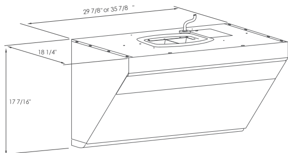
▲ Product Dimensions
