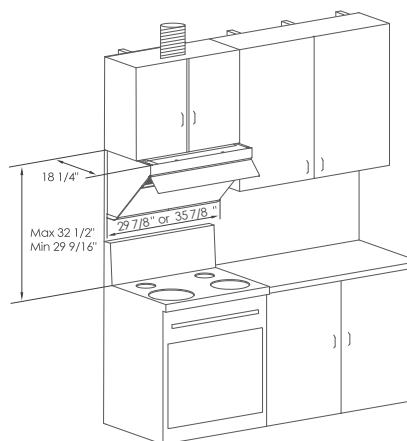
▲ Installation Dimensions
