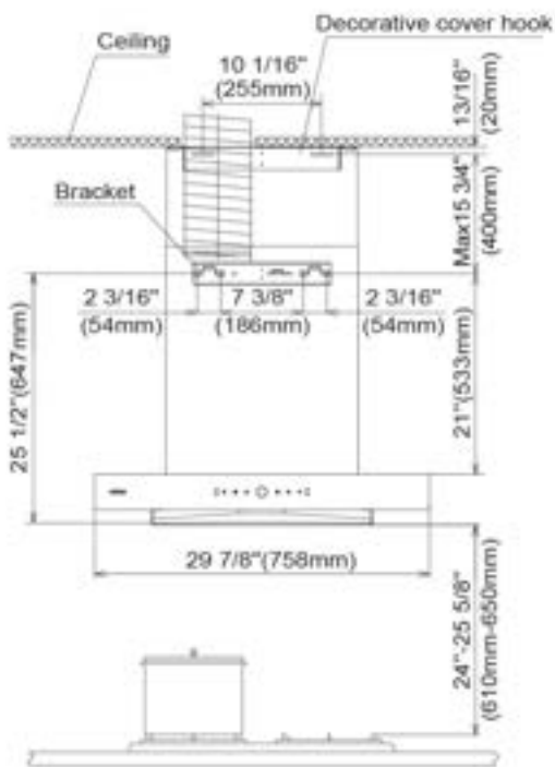
Wall-Mount Installation
