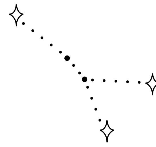
Cancer Constellation
