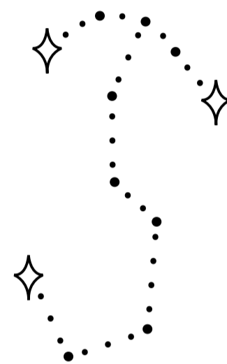
Scorpio Constellation
