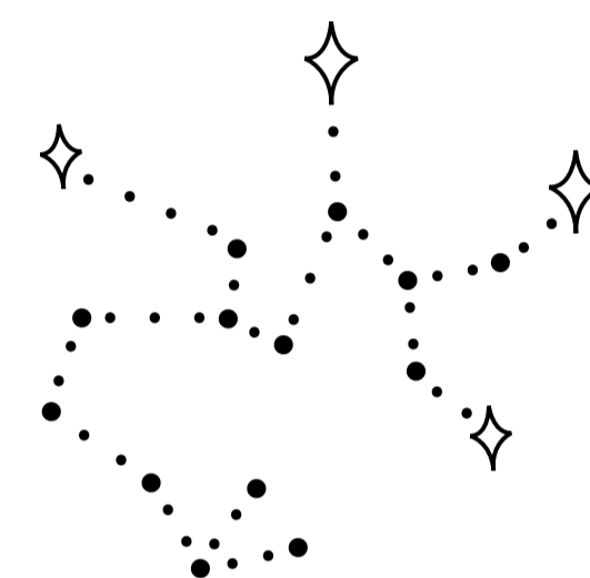
Sagittarius Constellation
