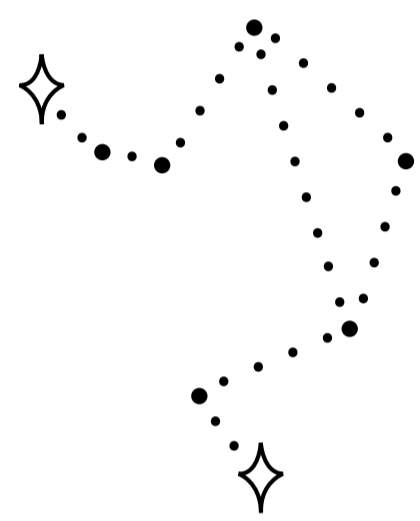
Libra Constellation
