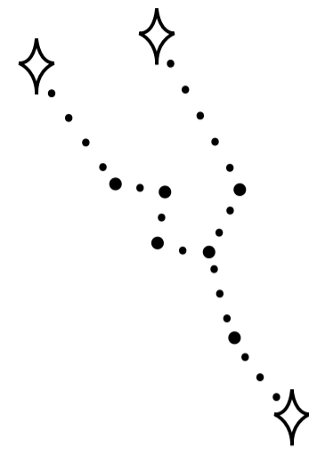
Taurus Constellation
