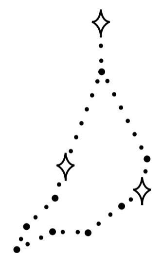
Capricorn Constellation
