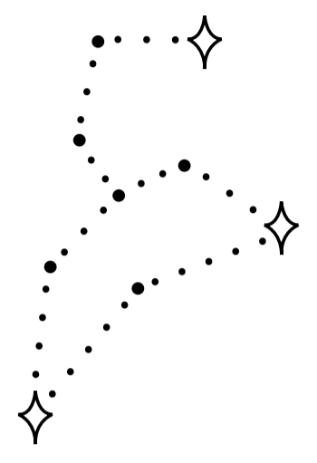
Leo Constellation
