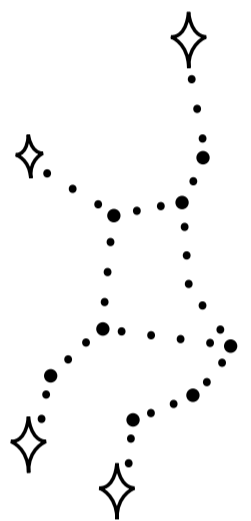
Virgo Constellation
