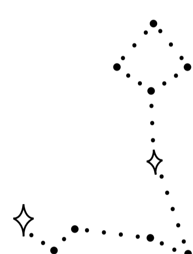
Pisces Constellation
