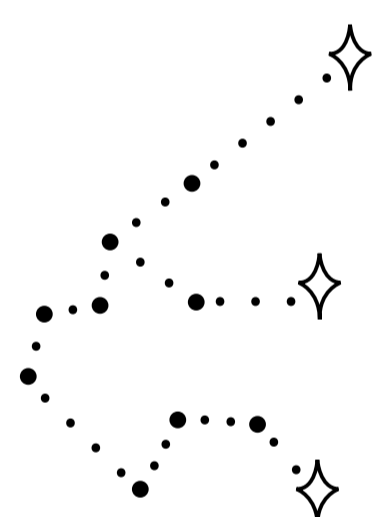
Aquarius Constellation
