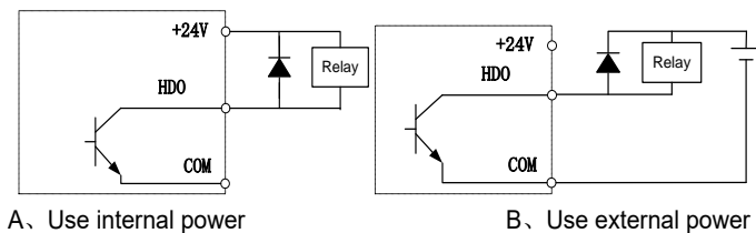
Figure 3-9 Wiring diagram of the switch output terminal
