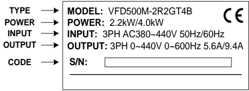
2-1 name plate
