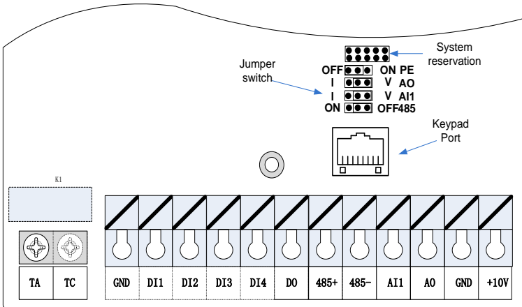
Figure 3-6 Schematic diagram of the VFD500M control circuit terminal (SIZE A)
