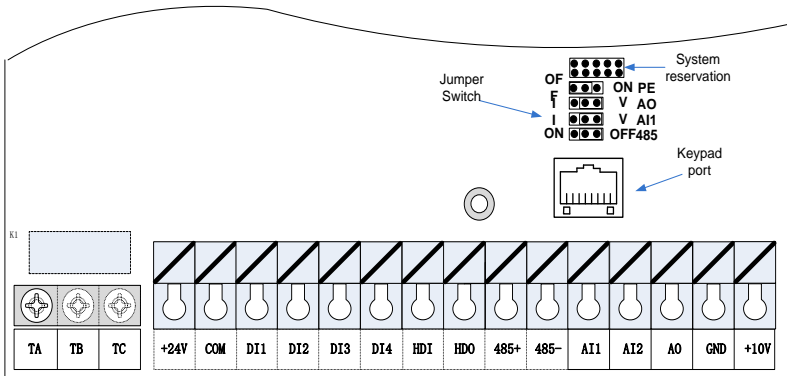
Figure 3-6 Schematic diagram of the VFD500M control circuit terminal (SIZE B/C)
