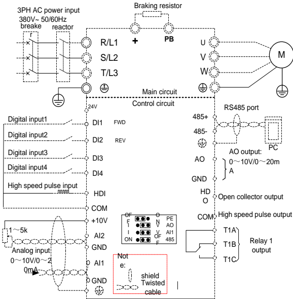
Figure 3-3 (SIZE B/C) standard wiring diagram
