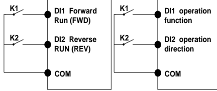
Figure1: Two-line mode 1
