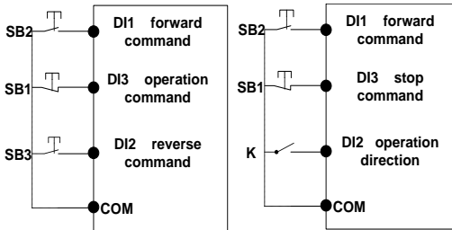
Figure 3: Three-line mode1
