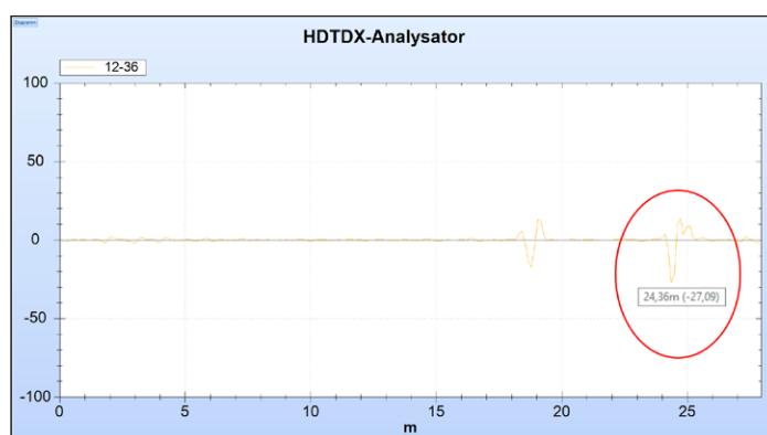
Cable tester ETHERtest V5.3
