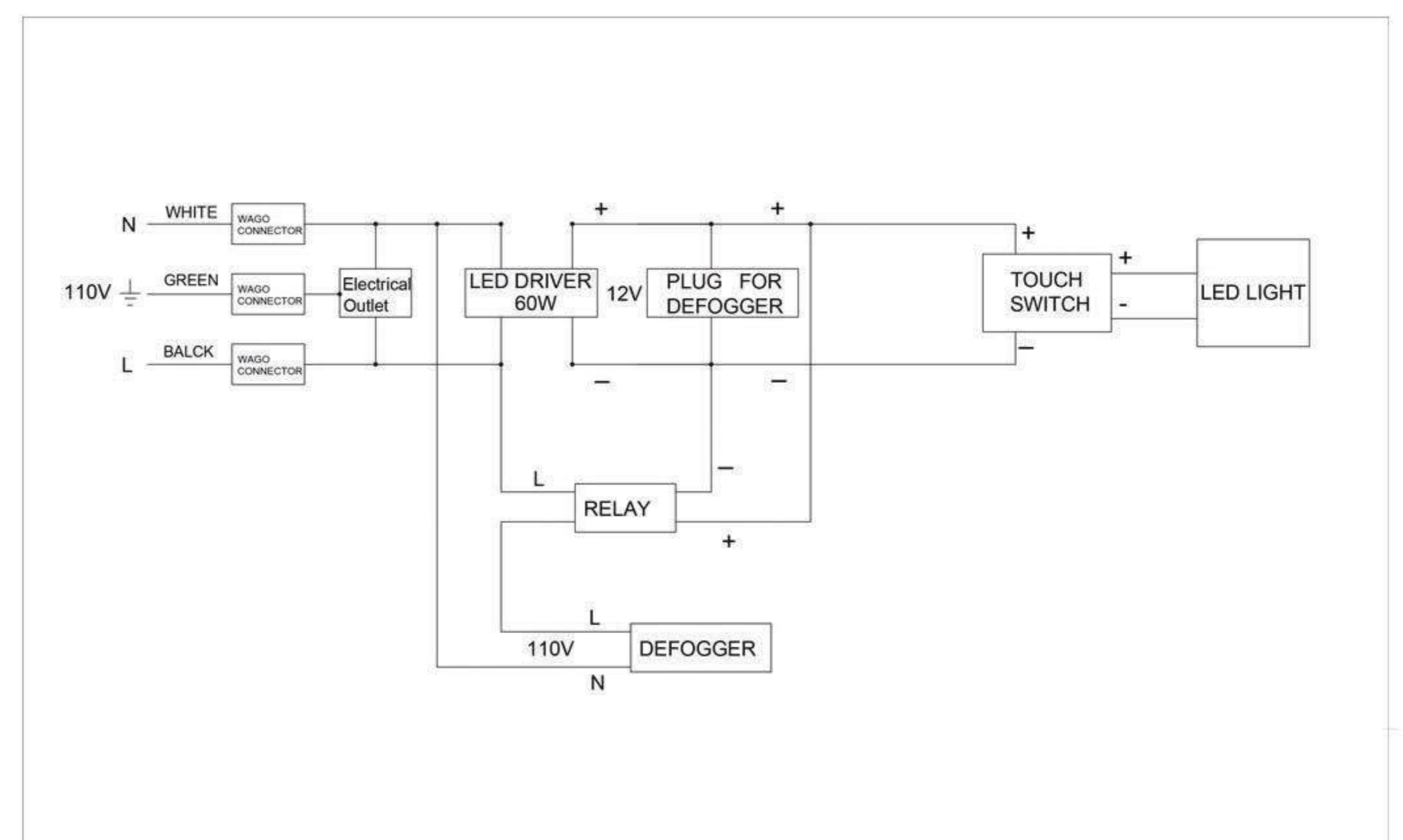
Circuit Diagram
