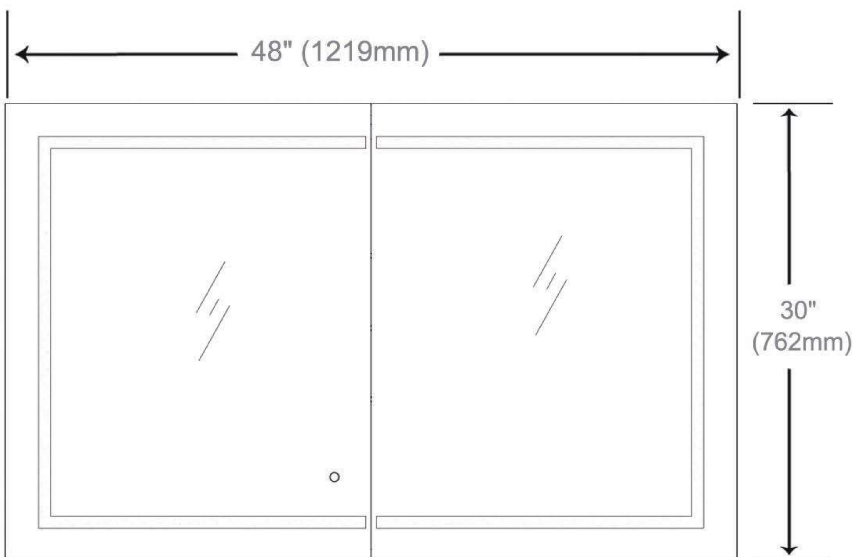
Cabinet Dimensions
