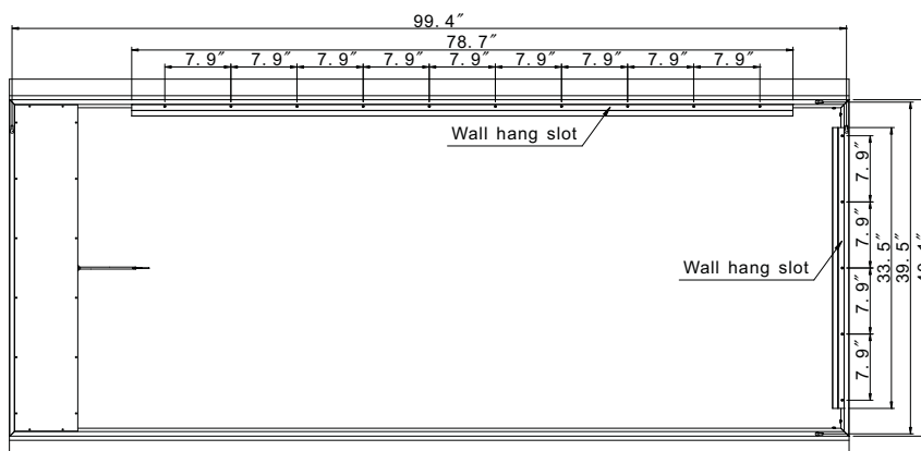
REAR VIEW
