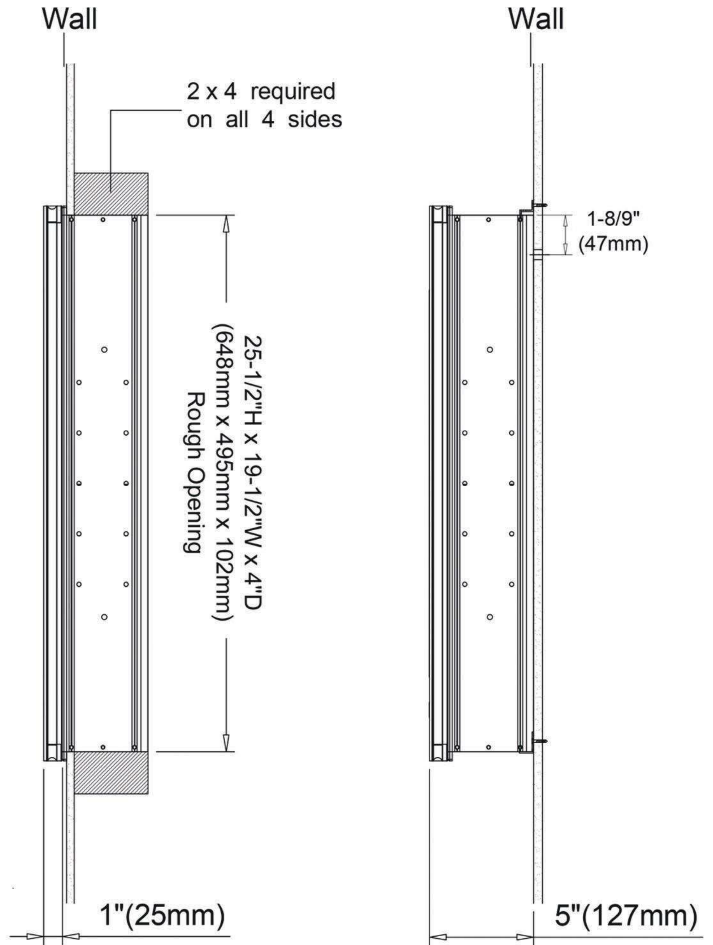
Recessed Mount
