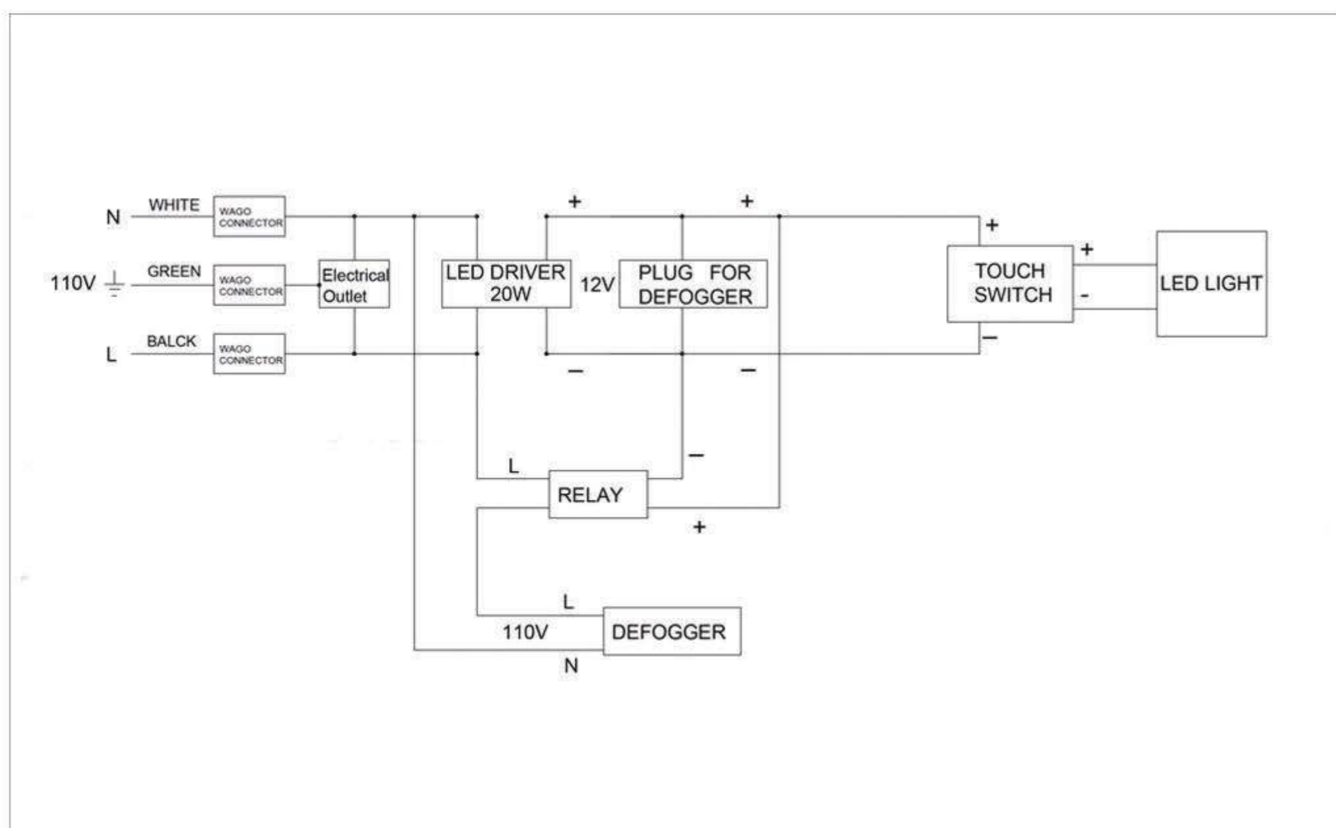
Circuit Diagram
