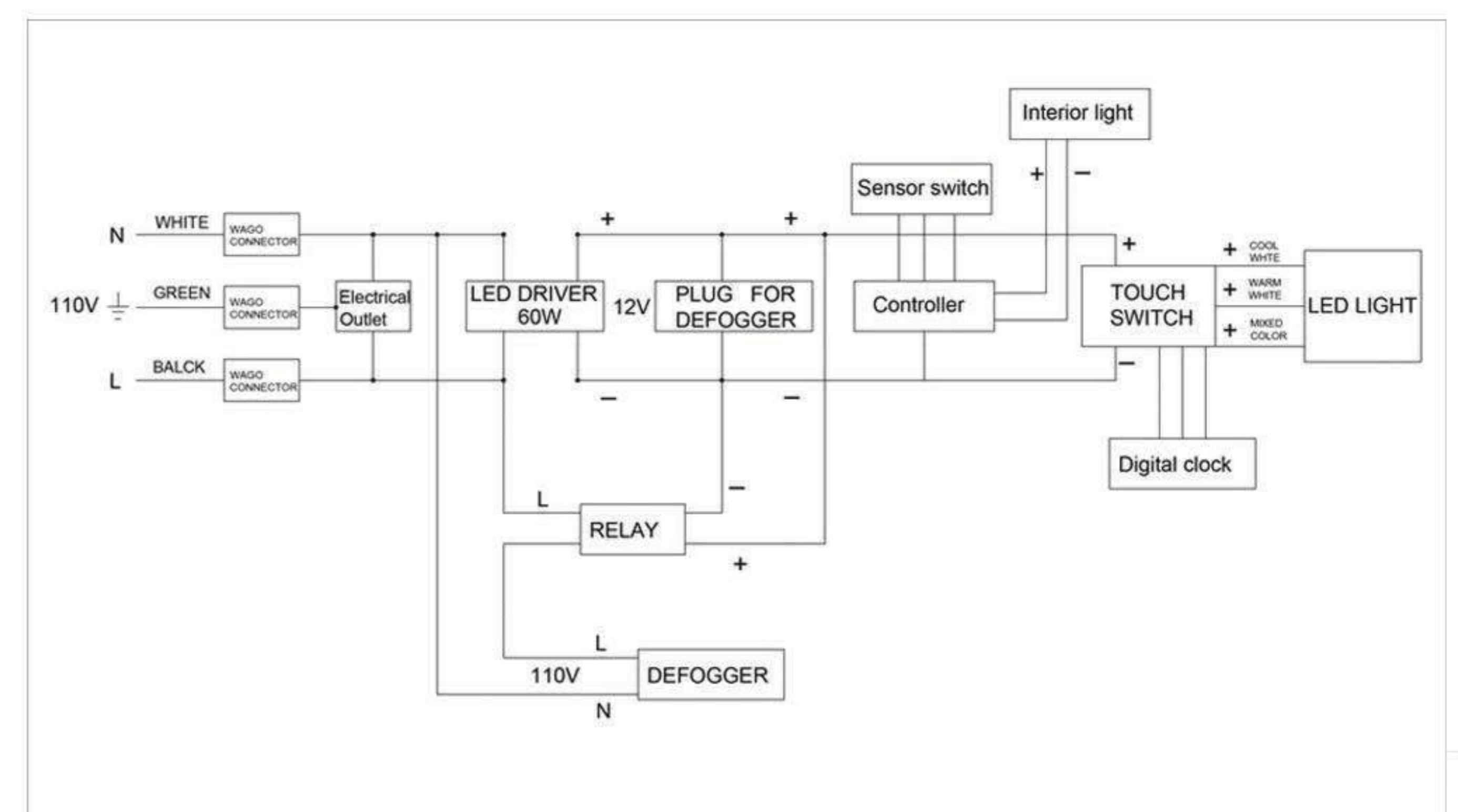
Circuit Diagram
