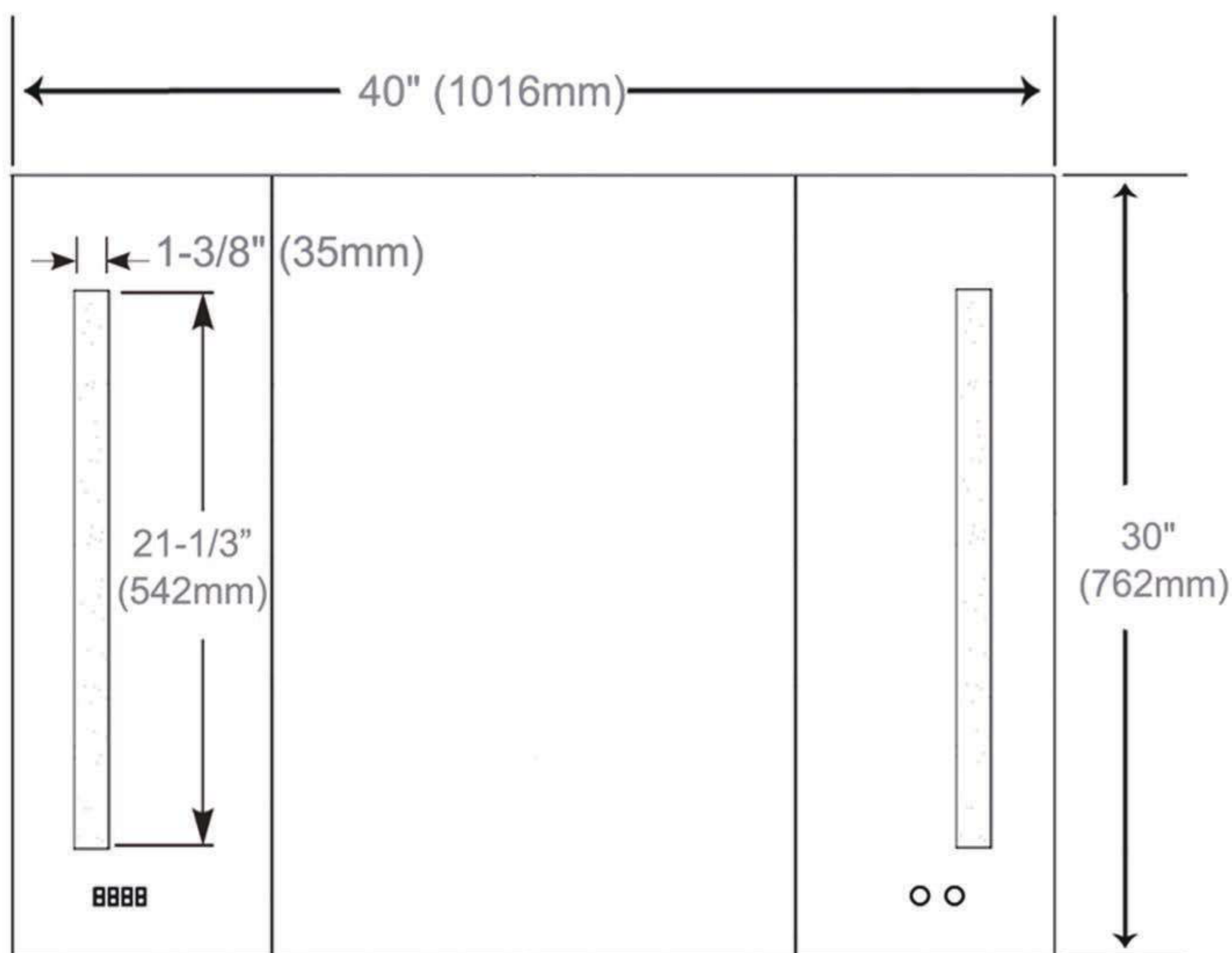
Cabinet Dimensions
