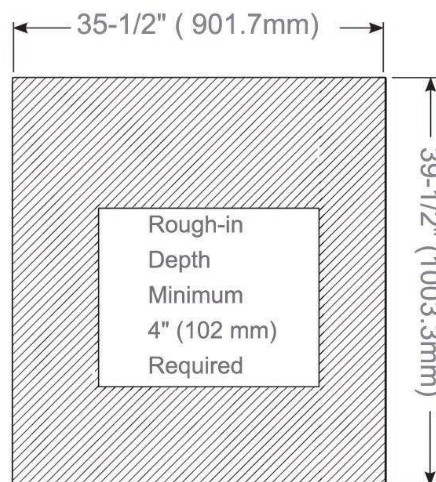
Rough-in Dimensions
