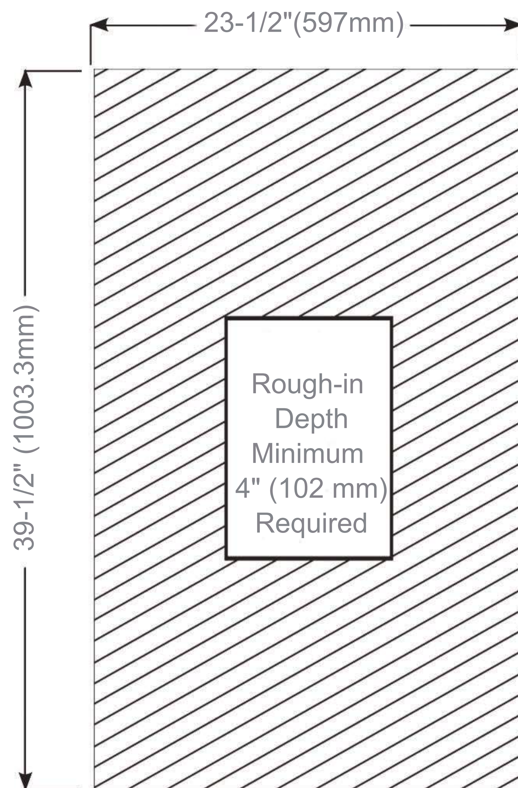
Rough-in Dimensions
