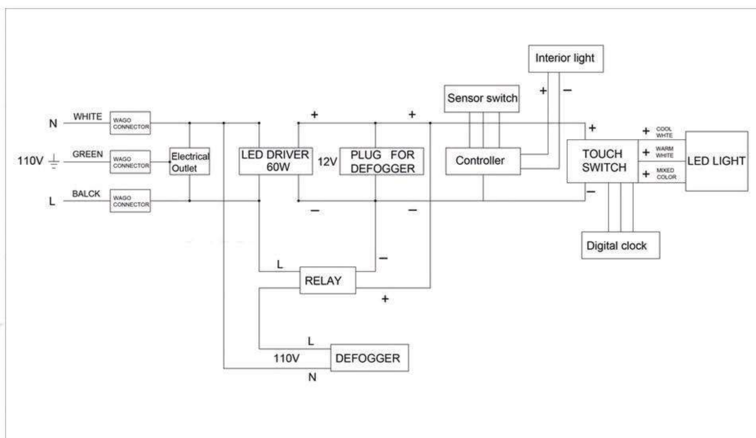
Circuit Diagram
