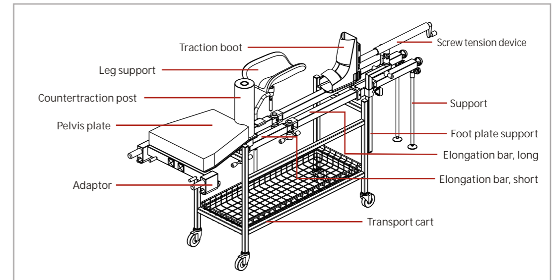
Orthopedics Extension 115-005691(005778 PU)-00
