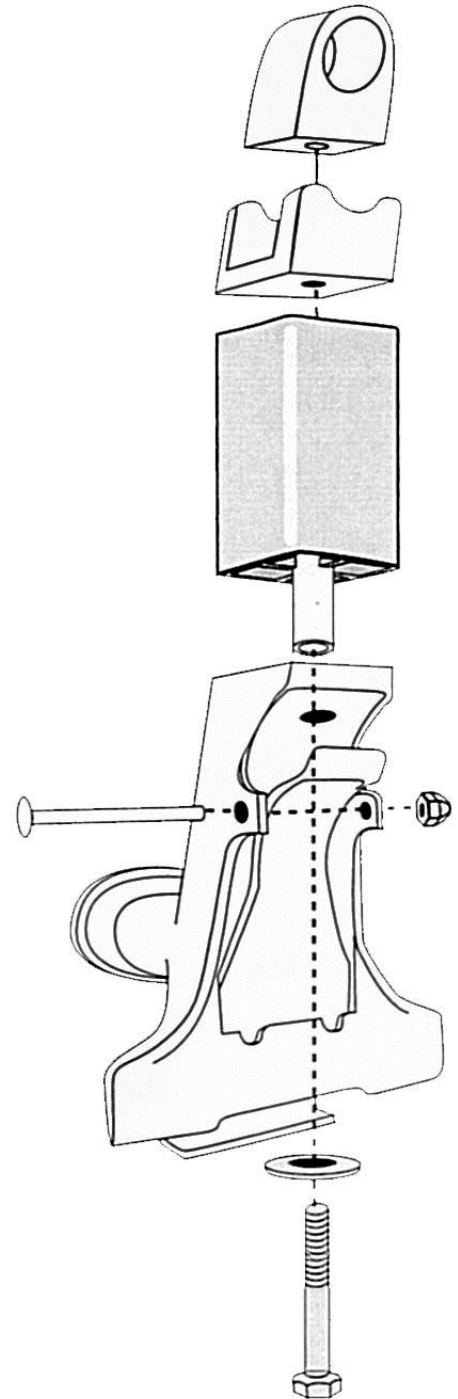
Figure 1: Raingutter Tower Exploded View
