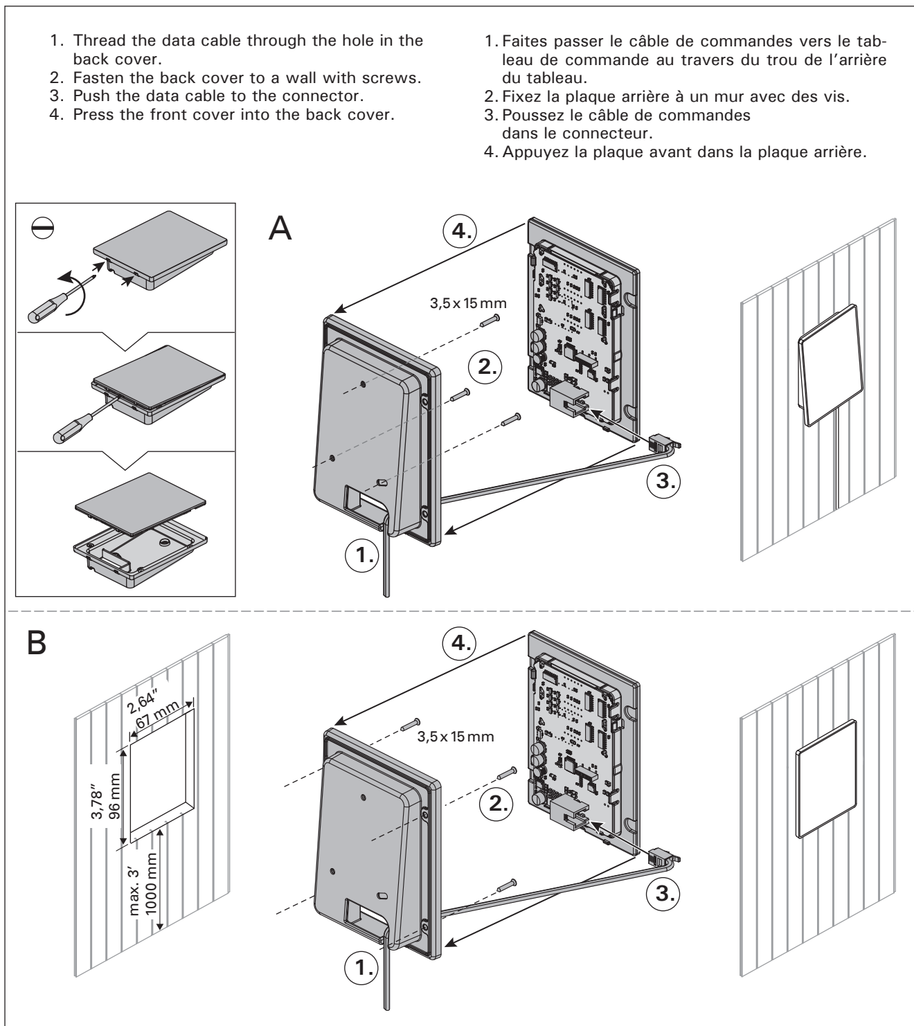
Figure 4. Fastening the control panel
