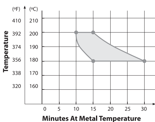
Typical Cure Cycle For Polyester
