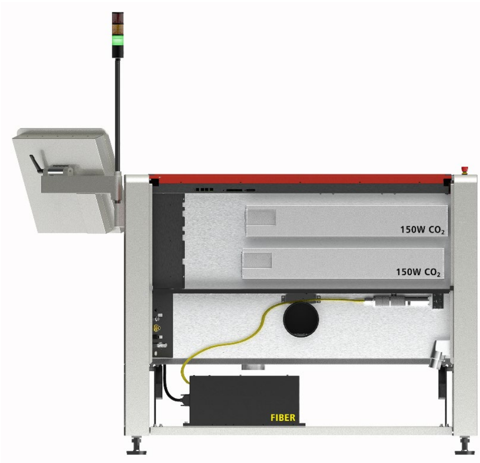
Multiple wavelength configuration with 300 watts CO 2 and 50 watts fiber
