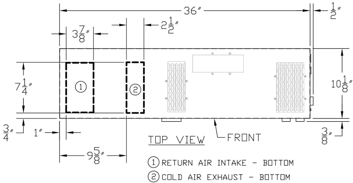
1800H ABOVE CELLAR COLD AIR CUTOUT DIMENSIONS
