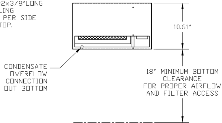
REAR VIEW
