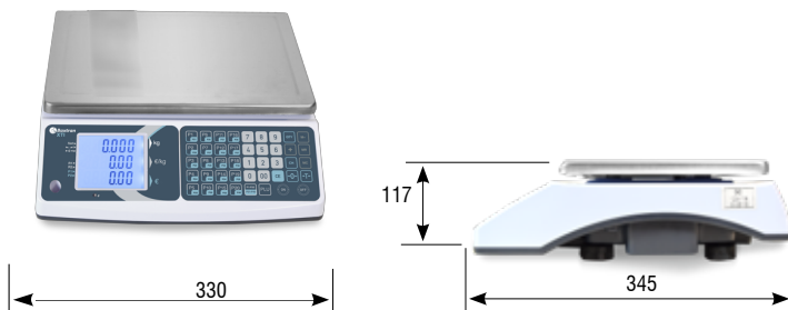
Dimensions (mm)
