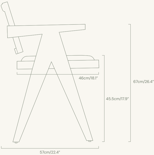
side profile
