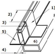
Figure1. Clamps (Clips) requirement 1) Clamp: Al alloy, 3 mm Min. thickness 2) Catch length (50 mm Min.) 3) Covering depth (7 mm Min. on the frame) 4) Supporting depth (10 mm Min.) 5) Frame (applicable to all frame sections) 6) Array rail (applicable to parallel or crossed mounting)
