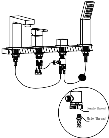
4. Fixed the switch and fasten the nut. Fix the converter handle by the hexagonal tool.
