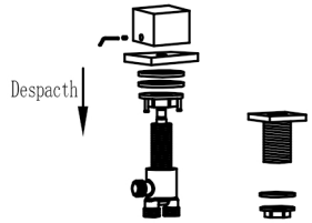
3. Take apart the handle and base by the hexagonal screwdriver. Take apart the nut and gasket of the shower holder.
