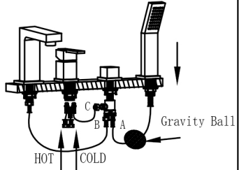
6. Pulling pipe connect with the conversion A through the shower holder. Gravity ball fixed on the top of the pull out pipe. Water nozzle connect to the conversion B, switch water outlet connect to the connector C and finally contact to the hot and cold water hose.
