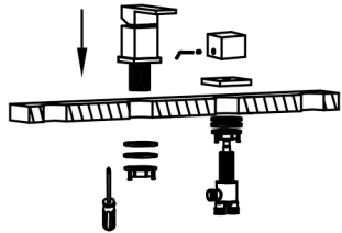
4. Fixed the switch and fasten the nut. Fix the converter handle by the hexagonal tool.
