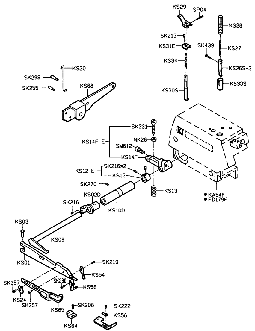
PARTS LIST FOR KS GROUP
