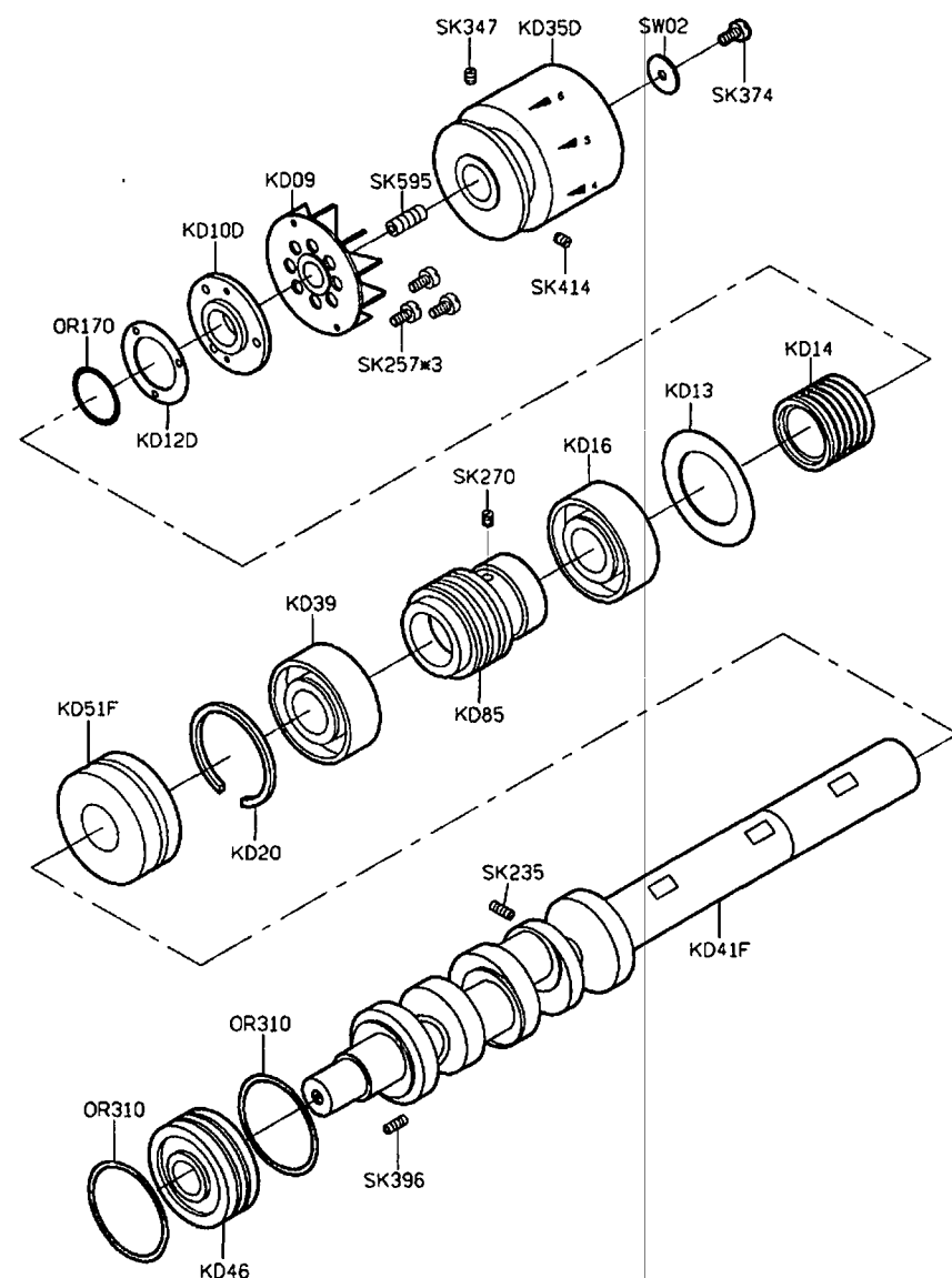
PARTS LIST FOR KD GROUP
