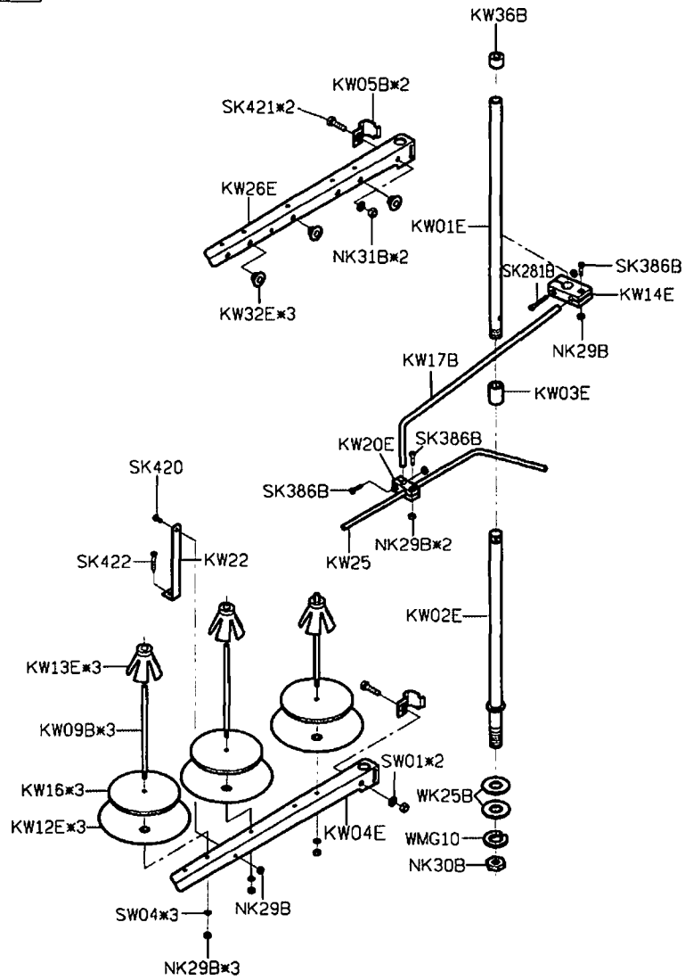
PARTS LIST FOR KW GROUP
