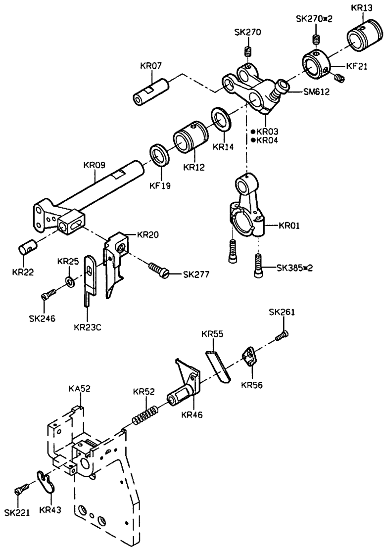
PARTS LIST FOR KR GROUP
