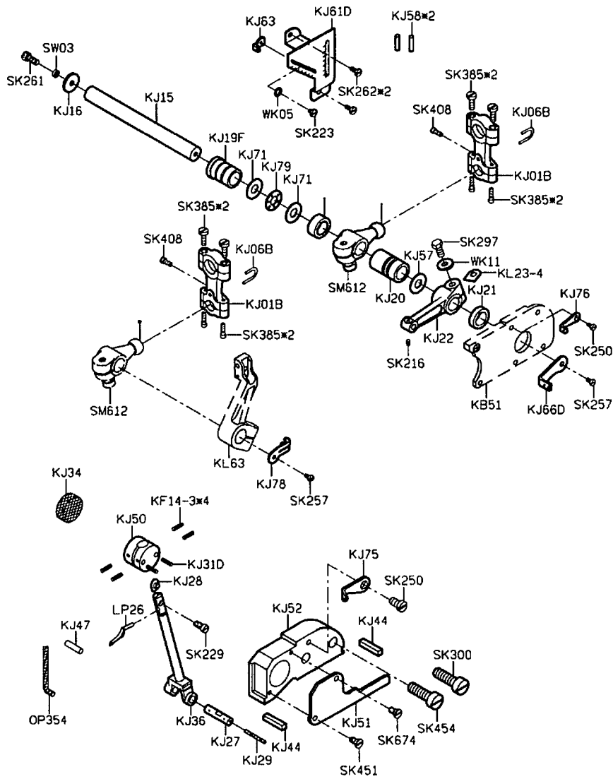
PARTS LIST FOR KJ GROUP
