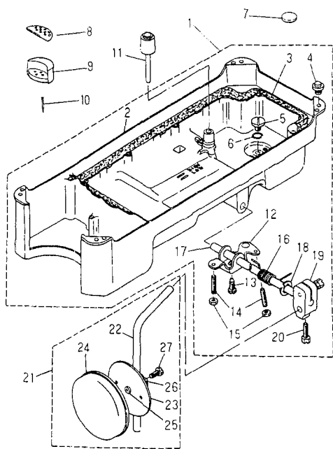
Oil reservoir & knee lifter components
