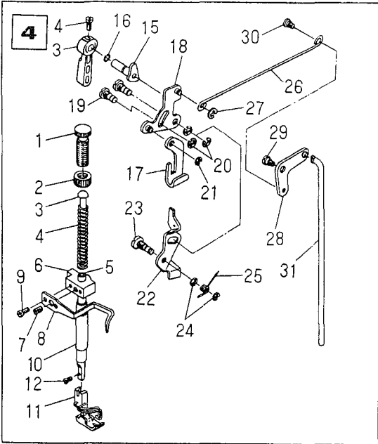
4. Presser bar components
