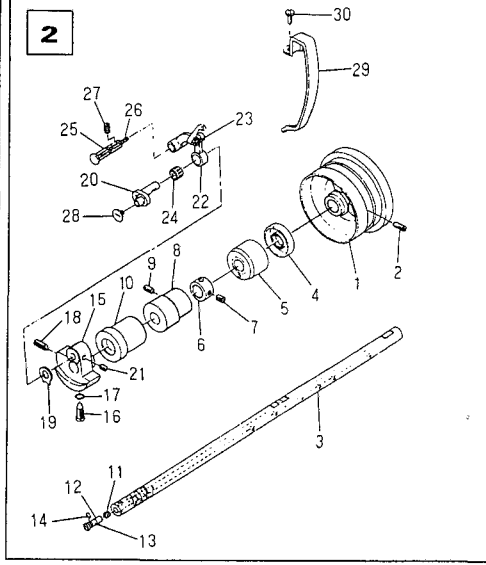
2. Main shaft & thread take-up components
