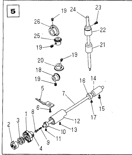
5. Hook driving shaft components
