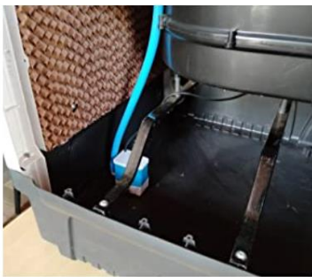
SEPARATE PUMP TO ENSURE BETTER WATER MOVEMENT - ENSURES BETTER COOLING
