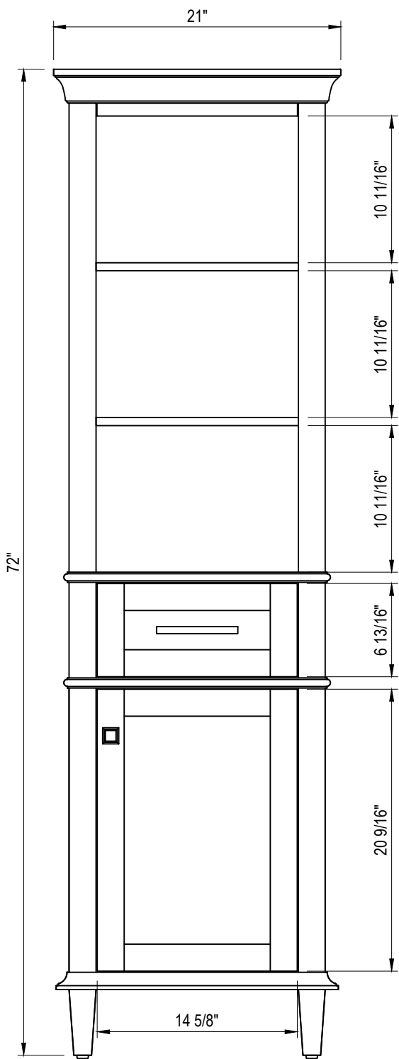
Front View
