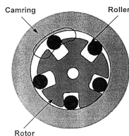
Roller Cell
