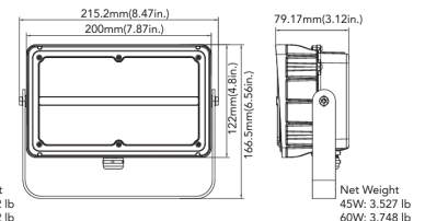
45W Trunnion Mount
