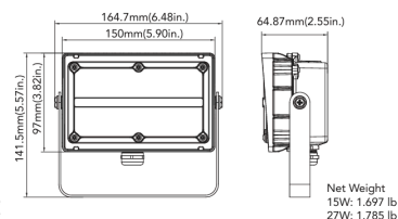
27W Trunnion Mount
