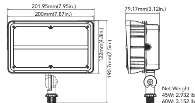
45W Knuckle Mount
