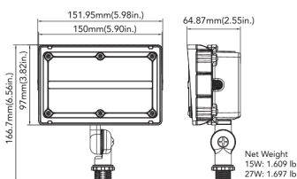
27W Knuckle Mount
