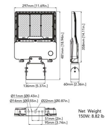
150W (Yoke Mount)
