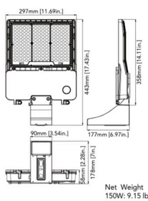
150W (Pole Mount)
