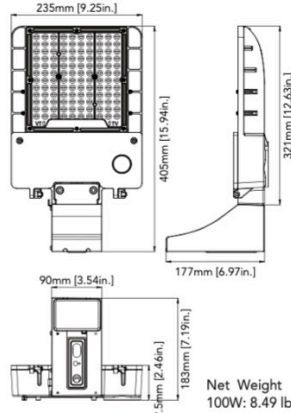
100W (Pole Mount)
