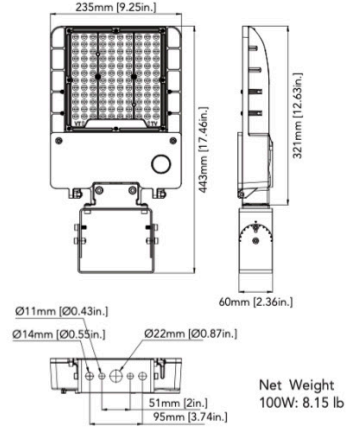
100W (Yoke Mount)
