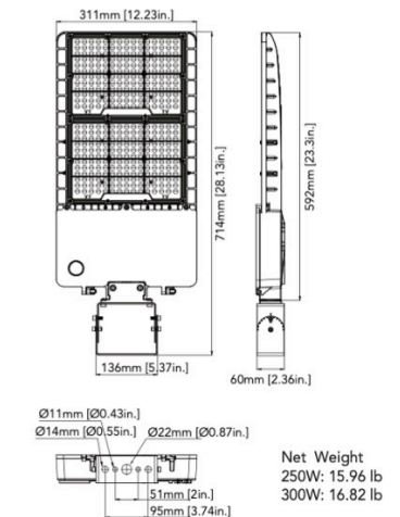
250W/300W (Yoke Mount)
