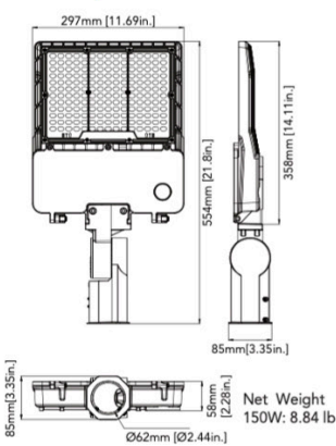
150W (Slipfitter Mount)
