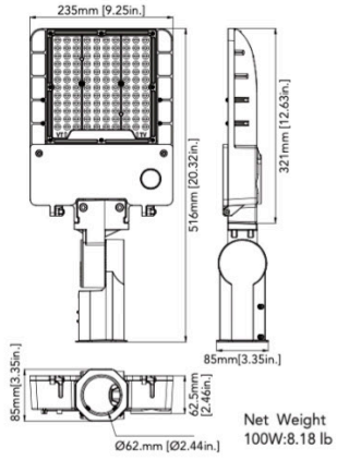
100W (Slipfitter Mount)
