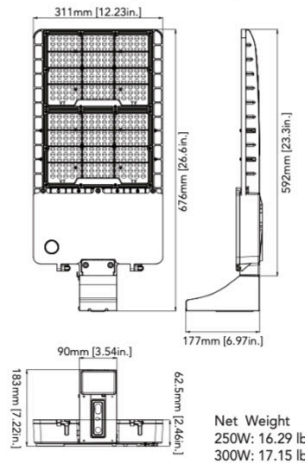
250W/300W (Pole Mount)
