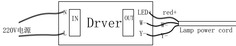
Schematic diagram of driving wiring
