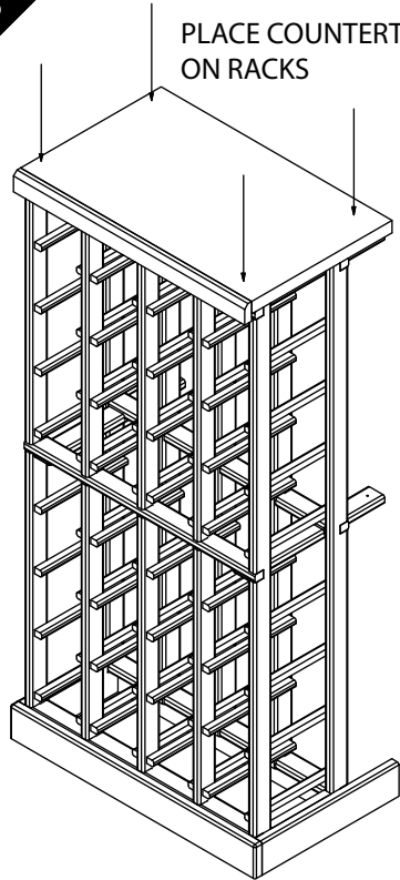
PLACING THE COUNTERTOP
