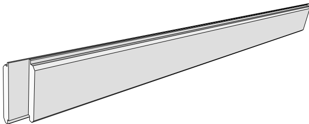
C1 (17x) 38x121x1380mm
