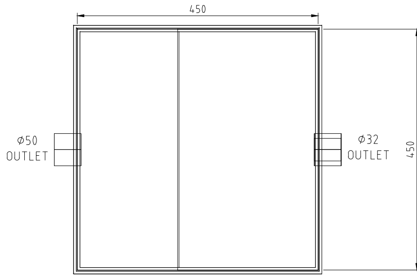
PLAN VIEW
