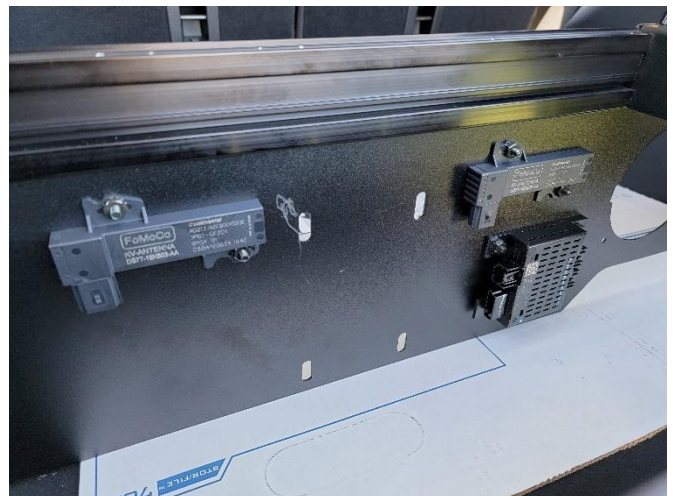
Install USB module and both key sense modules on inside of Havis console using supplied 10-32 x 1/2" machine screws and keps nuts.
