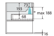
SIDE VIEW: DRAWER STORAGE
