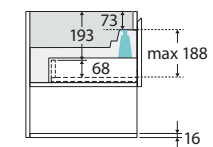
SIDE VIEW: DRAWER STORAGE
